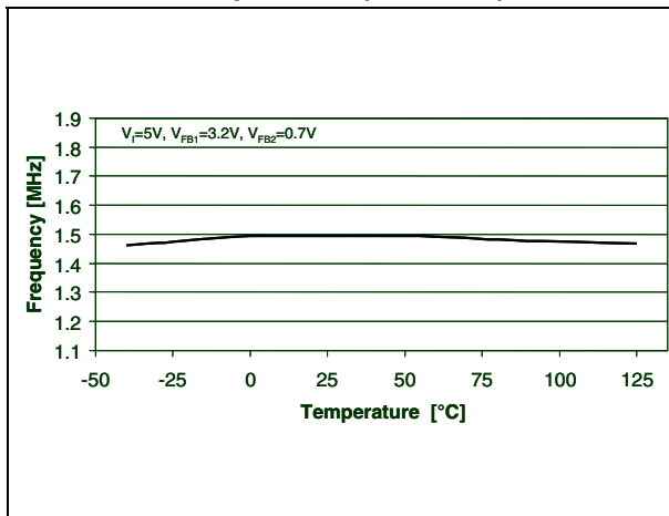
Figure 7. Switching frequency vs. temperature (ST2S06A)
